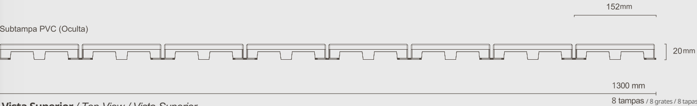
Vista Superior / Top View / Vista Superior
