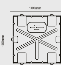
Vista Superior / Top View / Vista Superior
