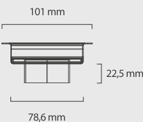
Vista Lateral / Side View / Vista Lateral
