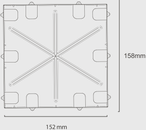
Vista Superior / Top View / Vista Superior
